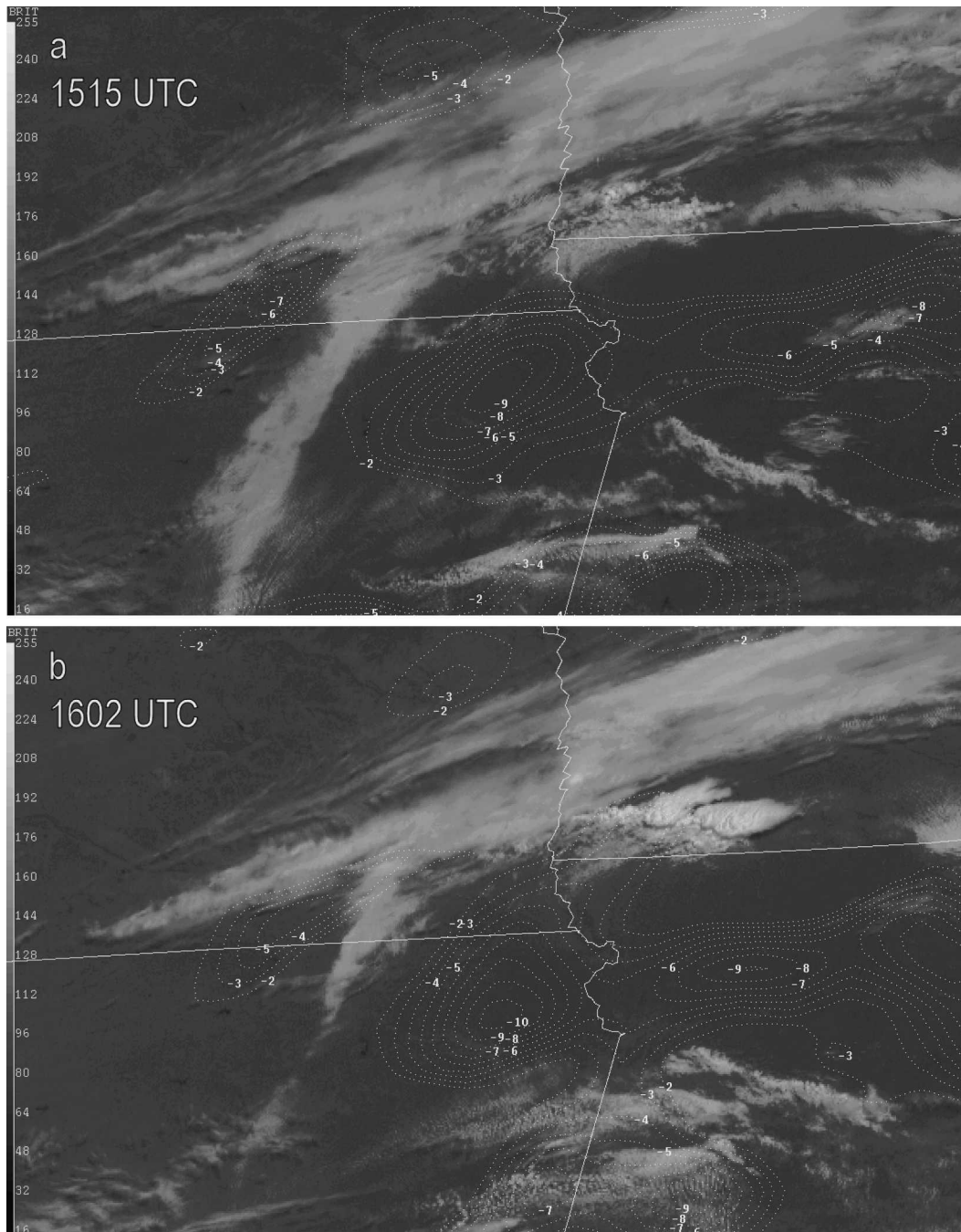
FIG. 4. GOES-12 1-km visible satellite imagery for 27 May 2004: (a) 1515 and (b) 1602 UTC. Surface moisture flux convergence (dotted lines, 10^{-4} \text{ g kg}^{-1} \text{ s}^{-1} , negative values only) from SPC surface objective analysis (Bothwell et al. 2002) at (a) 1500 and (b) 1600 UTC.
