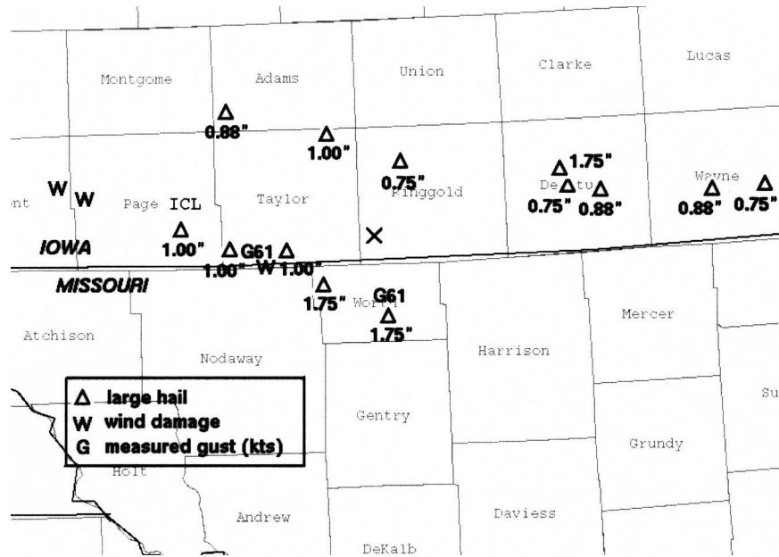
FIG. 6. Preliminary National Weather Service storm report data for 1600–1900 UTC 27 May 2004 across northern Missouri and southern Iowa. Location of RUC sounding in Figs. 5c and 5d is denoted by “X” in southwestern Ringgold County, IA. Clarinda, IA, is denoted by ICL. County borders are indicated by the gray lines with county names listed within.
