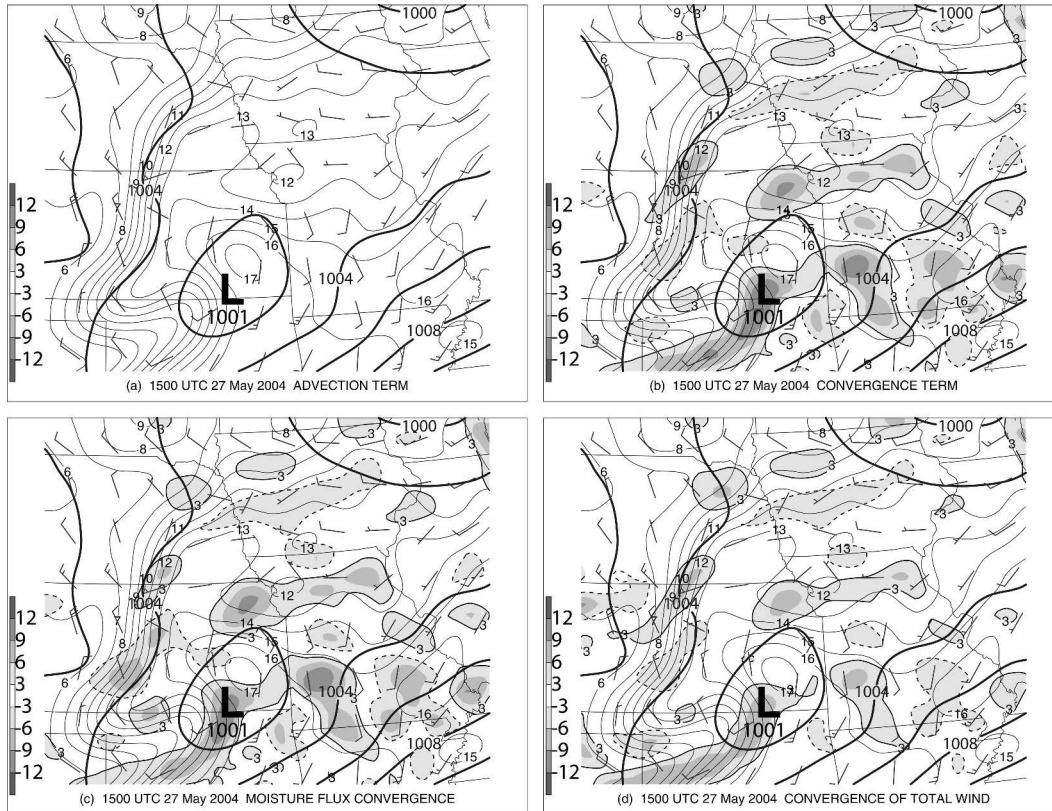
FIG. 3. As in Fig. 1, except for 1500 UTC 27 May 2004, and specific humidity contour interval is 1 \text{ g kg}^{-1} .
