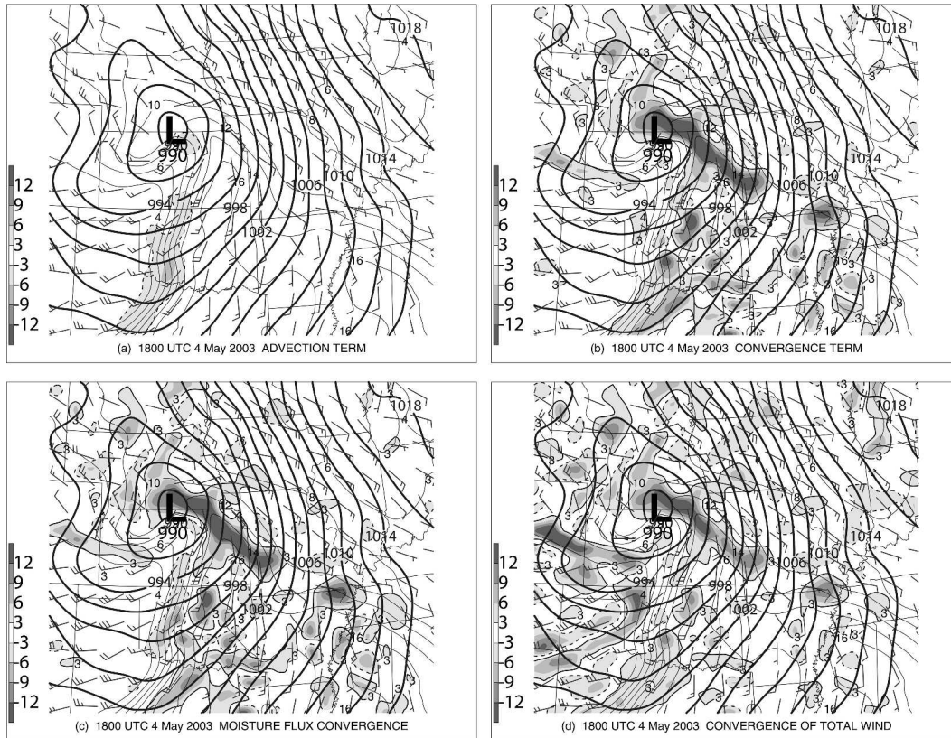
FIG. 1. Surface objective analysis valid at 1800 UTC 4 May 2003. Sea level pressure (thick solid lines every 2 mb), specific humidity (thin solid lines every 2 \text{ g kg}^{-1} ). Shaded regions represent (a) the advection term in MFC expression ( 10^{-4} \text{ g kg}^{-1} \text{ s}^{-1} ), where positive values represent moist advection; (b) the convergence term in MFC expression ( 10^{-4} \text{ g kg}^{-1} \text{ s}^{-1} ), where positive values represent convergence; (c) the total moisture flux convergence ( 10^{-4} \text{ g kg}^{-1} \text{ s}^{-1} ), where positive values represent positive MFC; and (d) the horizontal mass convergence of the total wind ( 10^{-5} \text{ s}^{-1} ), where negative values represent horizontal mass divergence. Thin dashed lines (thin solid lines) delineate negative (positive) values associated with shaded regions for each panel. Pennant, barb, and half barb represent wind speeds of 25, 5, and 2.5 \text{ m s}^{-1} , respectively.
