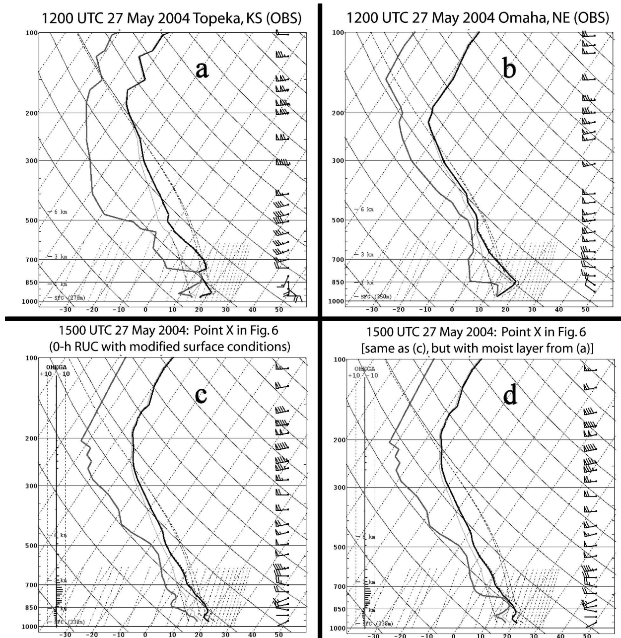
FIG. 5. Skew T - \log p plots of observed temperature (dark gray lines) and dewpoint temperature (light gray lines) for 1200 UTC 27 May 2004: (a) Topeka, KS, and (b) Omaha, NE. (c) RUC-2 0-h forecast sounding with modified surface conditions valid 1500 UTC 27 May 2004 near the Missouri/Iowa border (see "X" in Fig. 6 for location). (d) As in (c), except sounding is modified using low-level moist layer found on 1200 UTC Topeka sounding in (a). Horizontal bars represent vertical distribution of vertical motion ( \mu\text{b s}^{-1} ). Pennant, barb, and half barb represent wind speeds of 25, 5, and 2.5 \text{ m s}^{-1} , respectively.
